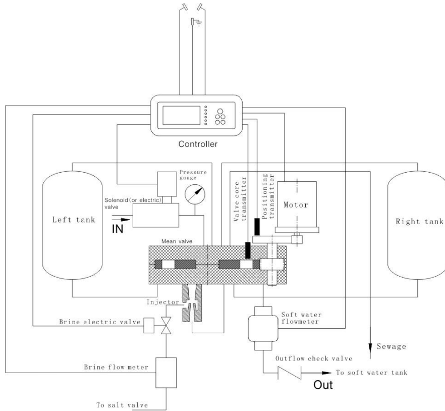
Picture 22:Control principle diagram
