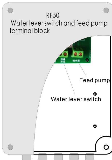
Picture11:RF50 Single contact water level switch terminal block
