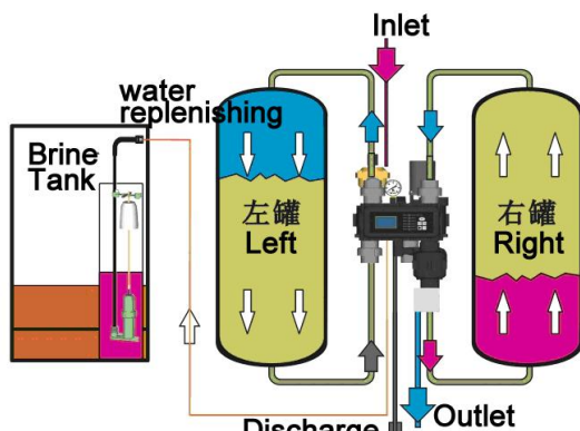
NO.5: Left tank cleaning; right tank outlet
