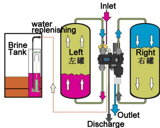
NO.1: Left tank outlet; right tank regeneration(Initiating) NO.2: Left tank outlet; right tank cleaning
