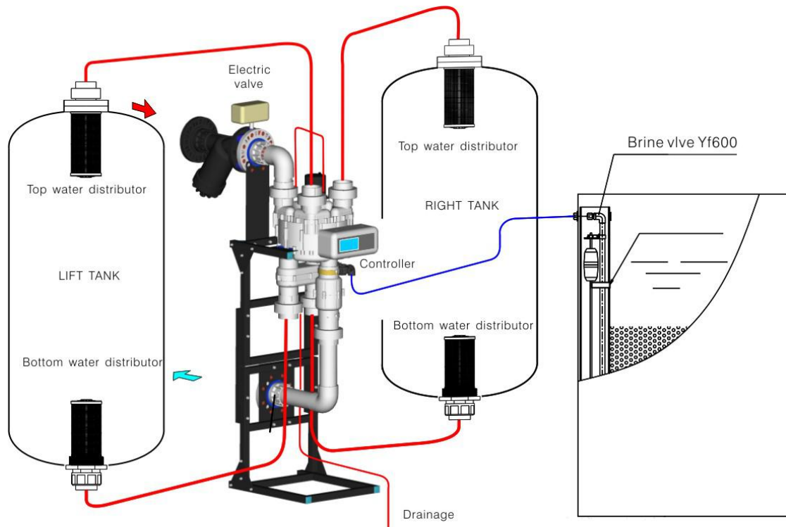
Picture 4: RF50 pipe install
