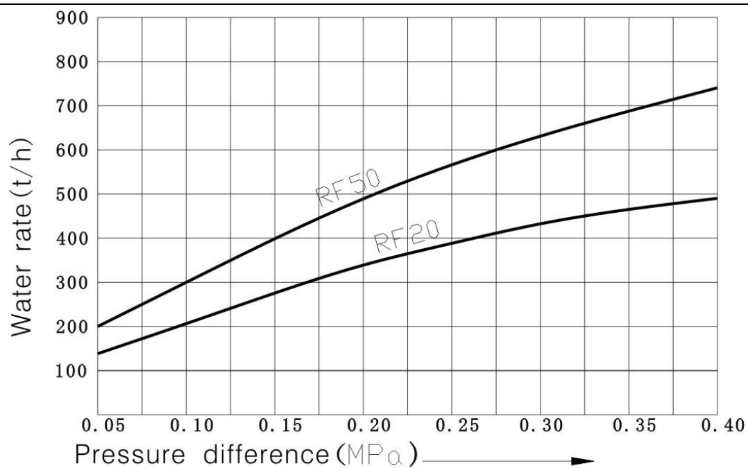
Picture 26: RF Brine flow pressure curve
