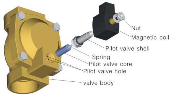
Picture :Repair picture of DF series solenoid valve
