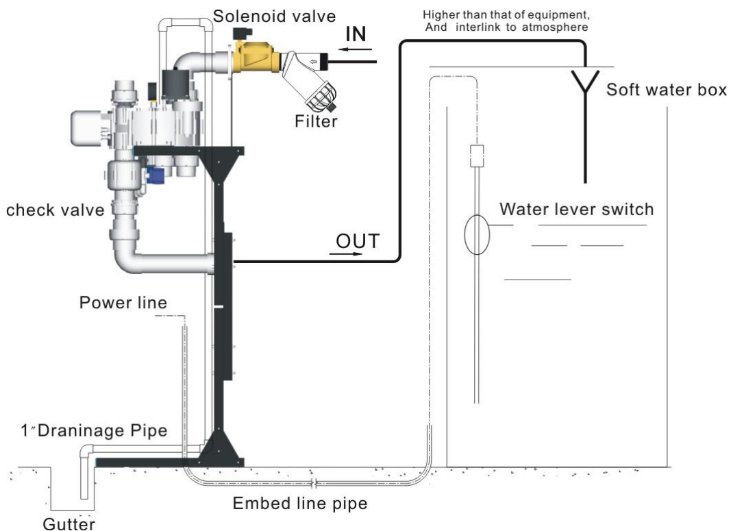
Picture 6: RF20 IN & OUT pipe install
