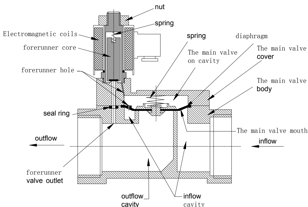
Picture14: Solenoid valve Principle
