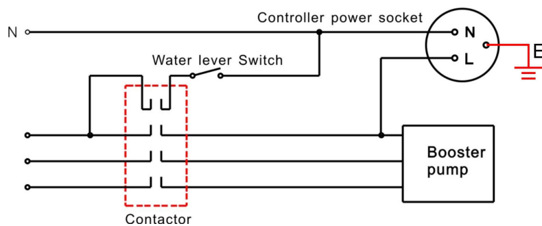
Picture 10: RF20 Single contact water level switch, the linkage of the feed water pump control
