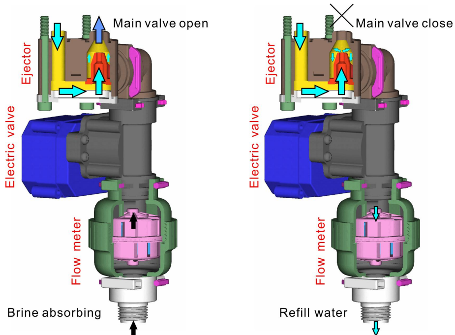
Picture17: Brine flow meter and electric valve system
