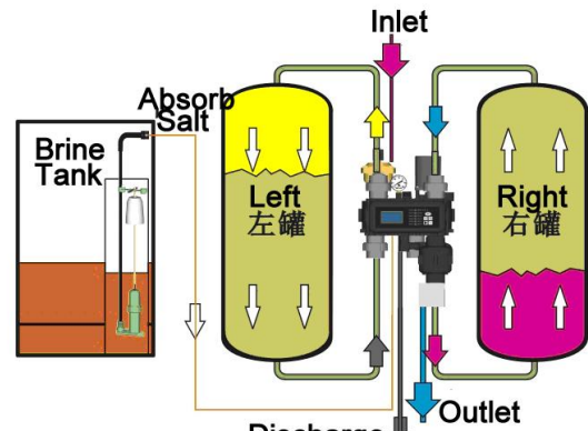
NO.4: Left tank regeneration; right tank outlet
