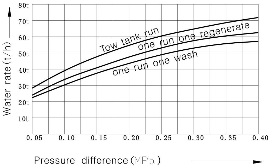
Picture 25: RF50 Flow pressure curve
