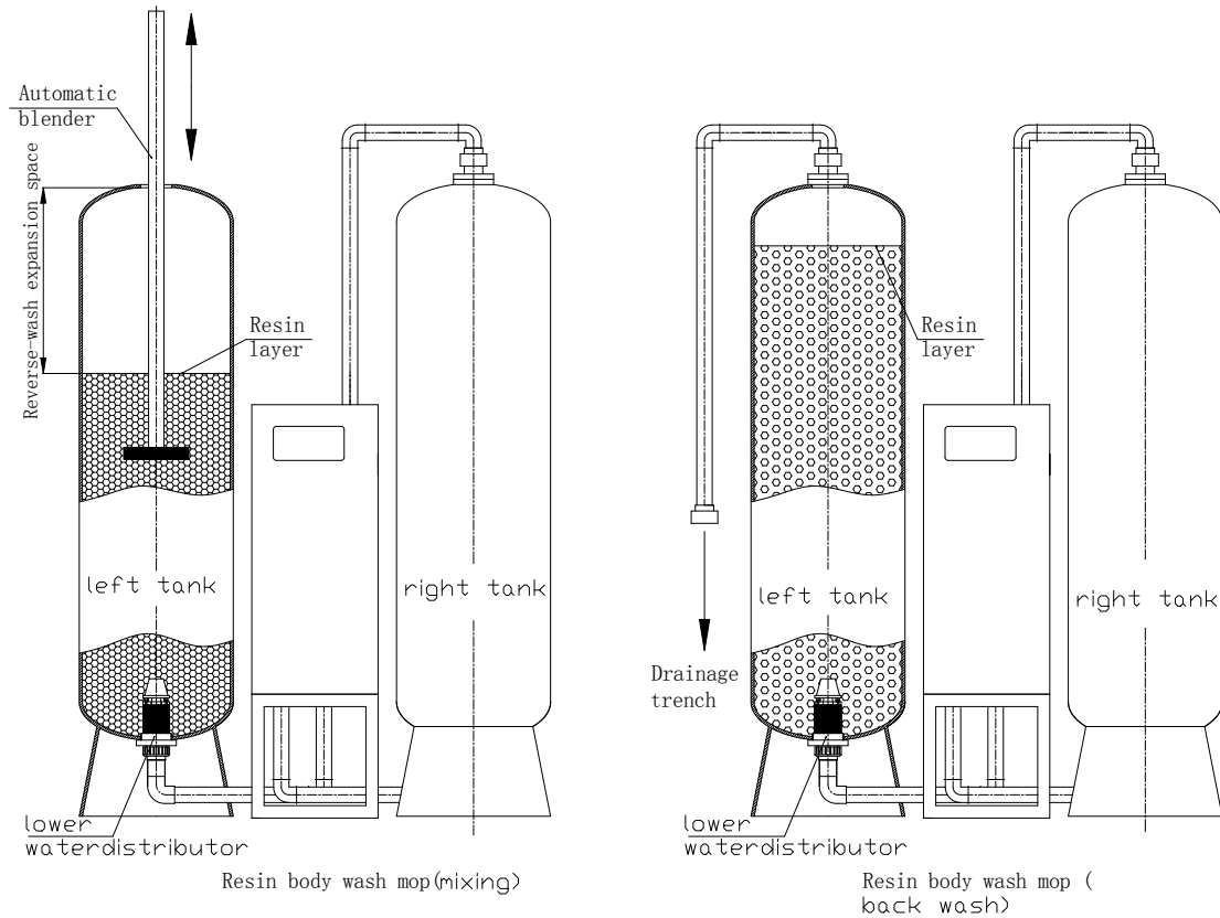
Picture16: Resin scrub
