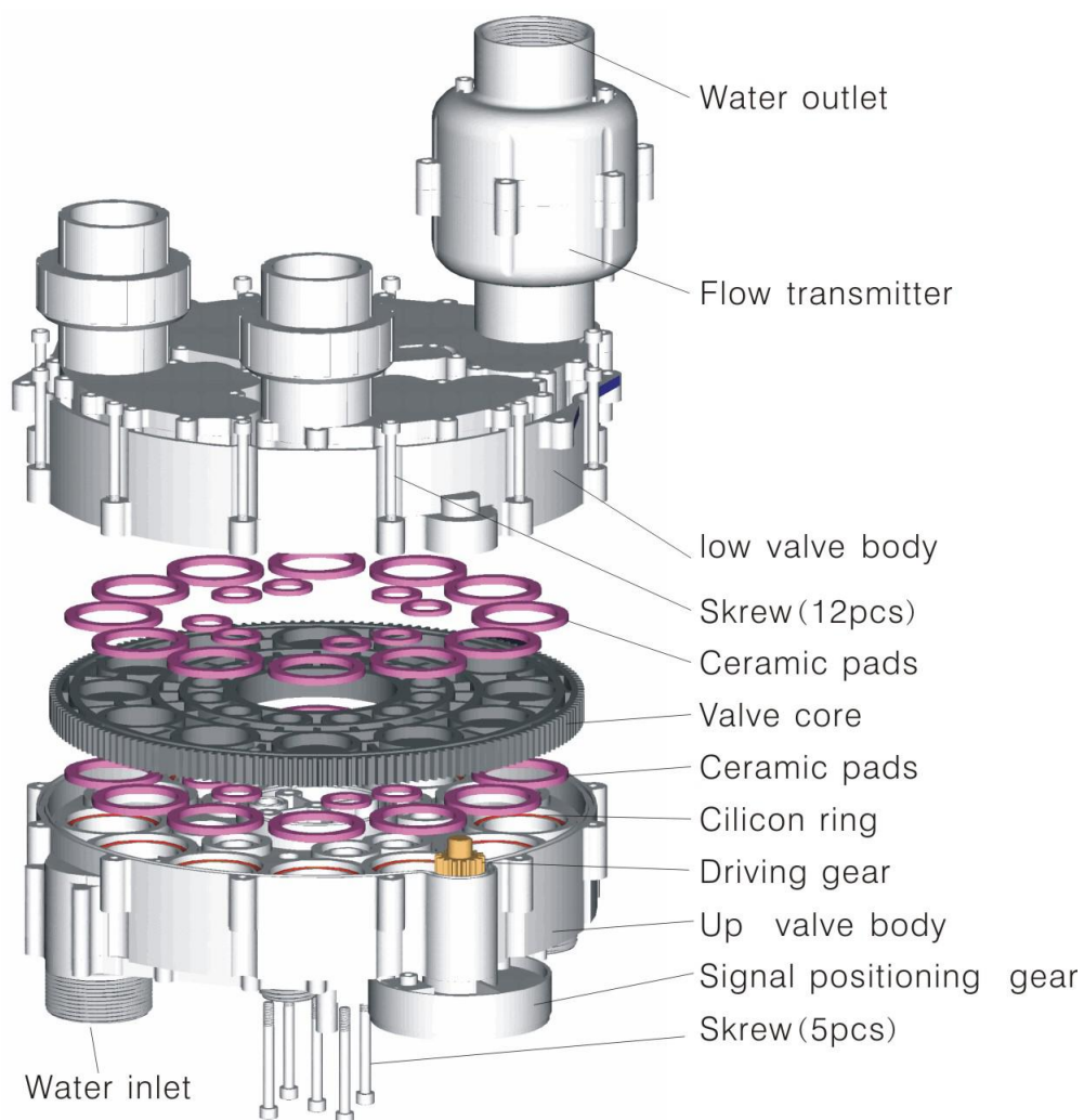
Picture19: Main valve exploded view
