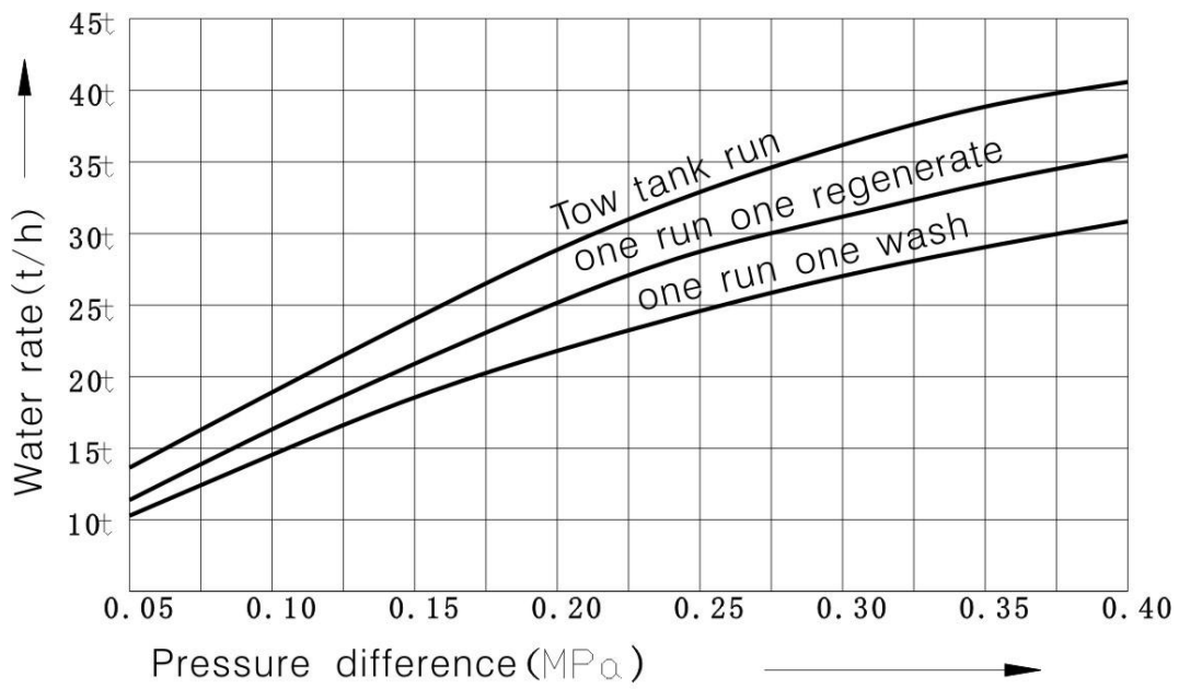
Picture 24:RF20 Flow pressure curve
