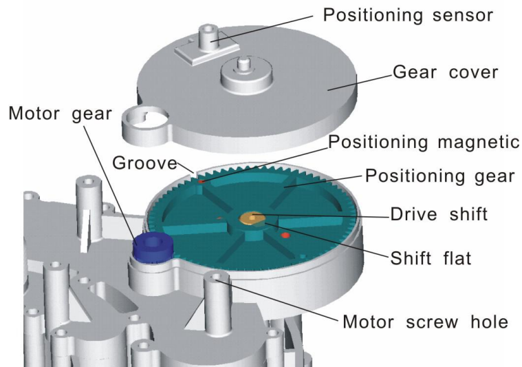
Picture 20: Position gear and drive system
