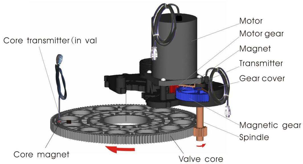
Picture18: multiple valve drive schematic
