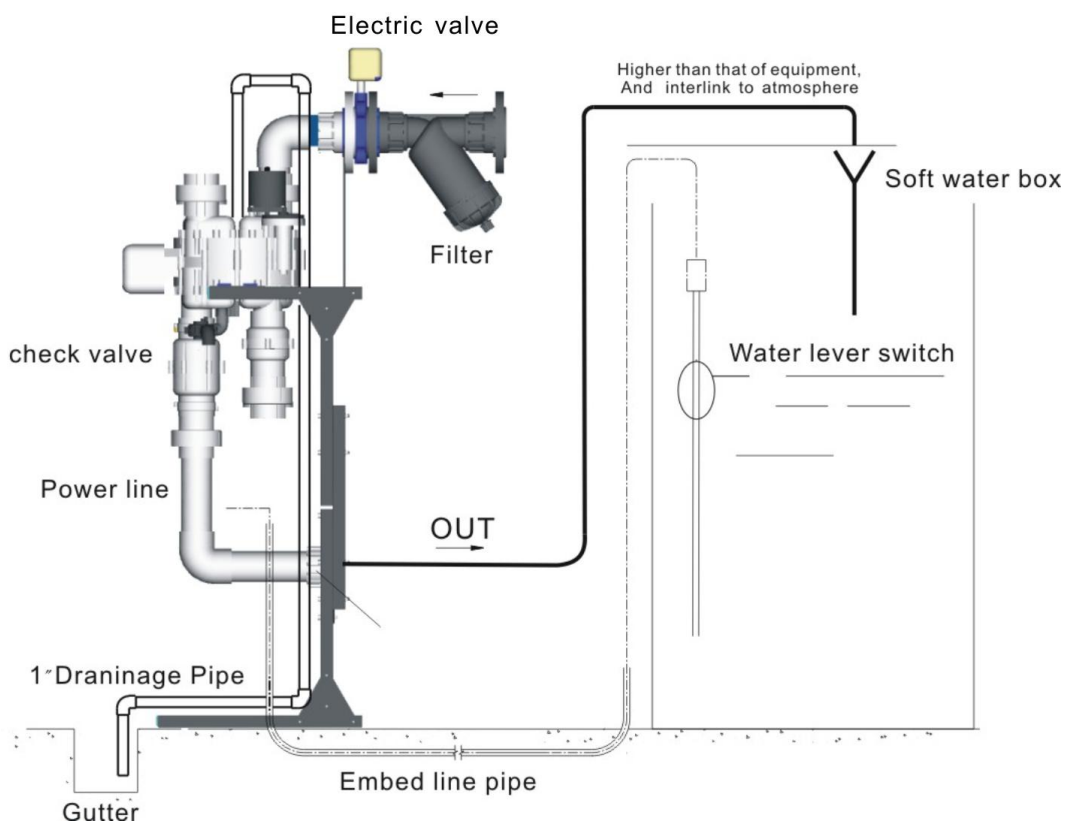
Picture 7: RF50 IN & OUT pipe install
