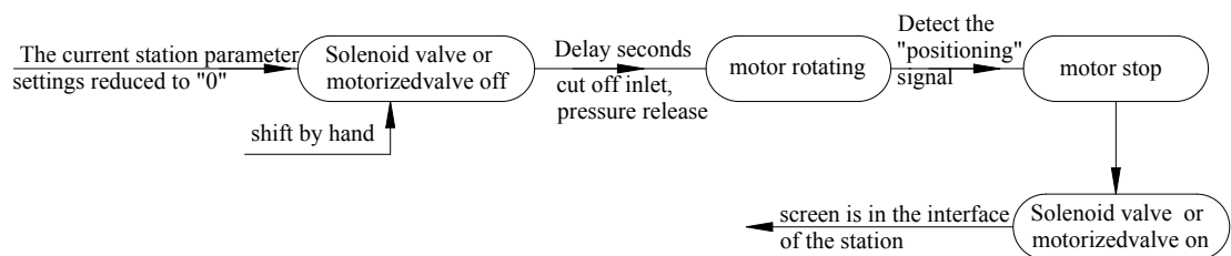
Picture 23:Main valve shifting procedure
